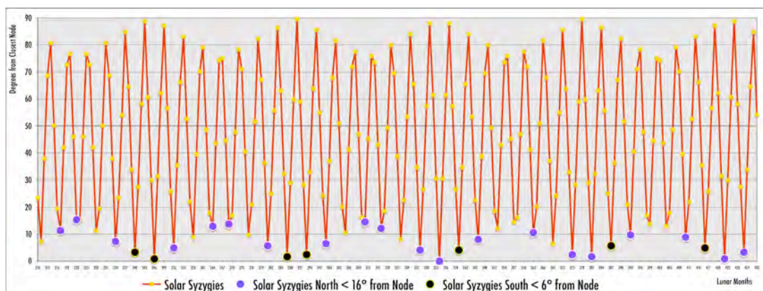
Supplementary Figure 19 | Graph for solar eclipses, showing degrees of elongation between syzygy and closest node. The model shows the effect of the asymmetrical criteria for syzgies North or South of the ecliptic. The irregular pattern of gaps implied by the index letters appears to apply to the solar predictions only.
